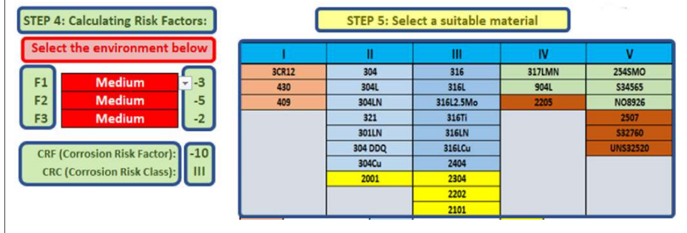
FIGURE 3 FINDING RISK FACTOR, CLASS, AND MATERIAL SELECTION
