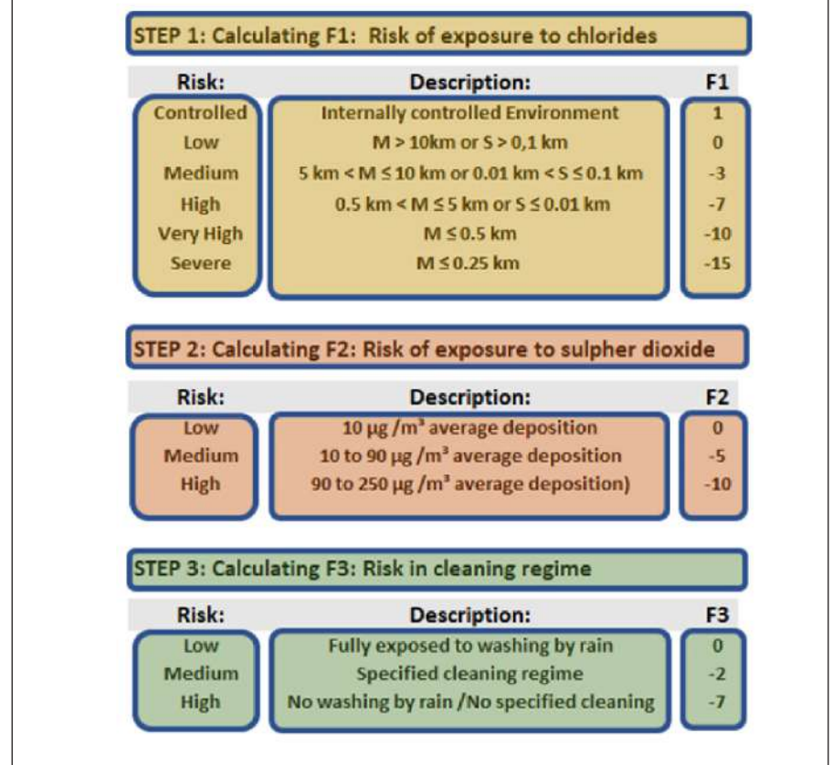
FIGURE 2 SELECTION OF F1, F2, AND F3
